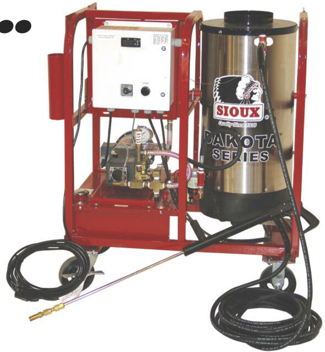
Model S1.5D250 Steam Cleaner 0.75 HP, 1.5 GPM, 250 PSI, Oil Fired
